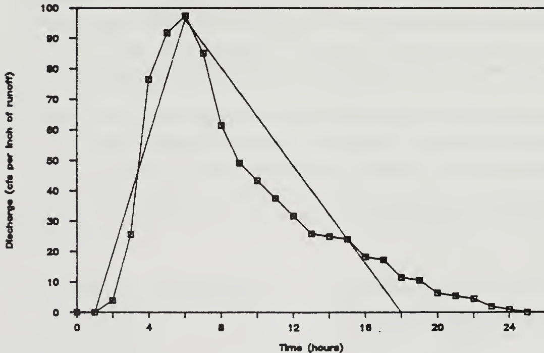
Figure 2. Unit hydrograph (2.5 hour effective storm duration) and approximated triangular unit hydrograph ( T_r/T_p = 2.40 ) for Deer Creek, Oregon Coast Range.
